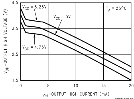
Receiver V_{OH} vs I_{OH} vs V_{CC}
