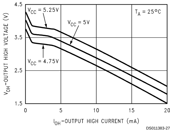
Receiver V_{OH} vs I_{OH} vs V_{CC}
