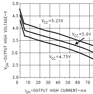
Driver V_{OH} vs I_{OH} vs V_{CC}
