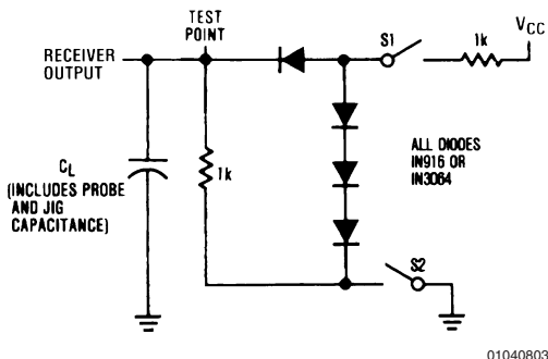
FIGURE 2. Receiver Propagation Delay Test Circuit
