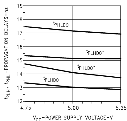
Driver Single-Ended Propagation Delay vs V CC
