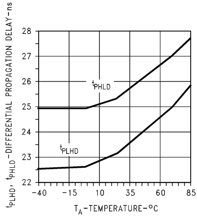
Receiver Differential Propagation Delay vs Temperature
