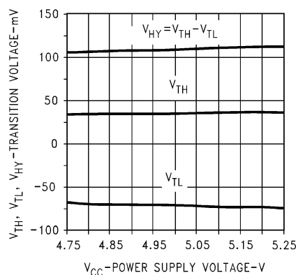
Hysteresis and Differential Transition Voltage vs V_{CC}
