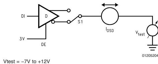
FIGURE 4. Driver I_{OD}
