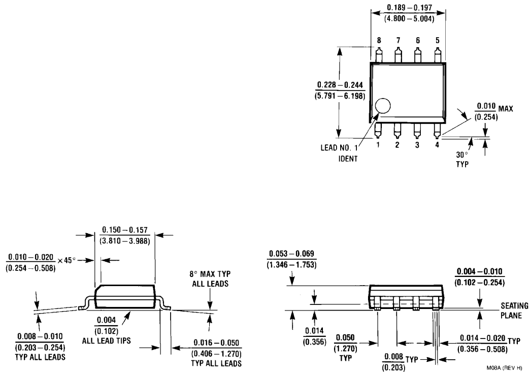
8-Lead (0.150" Wide) Molded Small Outline Package, JEDEC Order Number DS36C280M or DS36C280TM NS Package Number M08A
