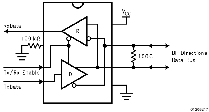
FIGURE 17. Typical Pin Connection
