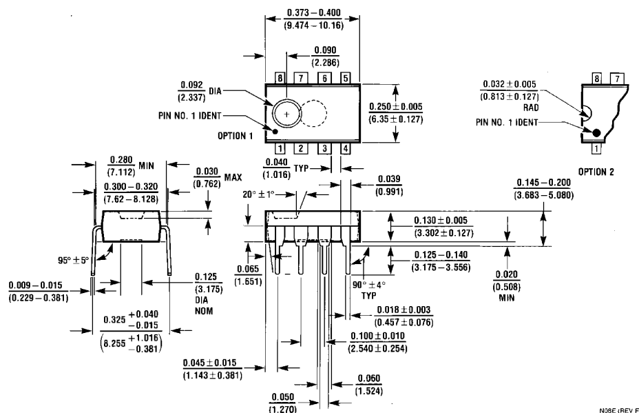
Molded Dual-In-Line Package (N) Order Number DS9638CN NS Package Number N08E
