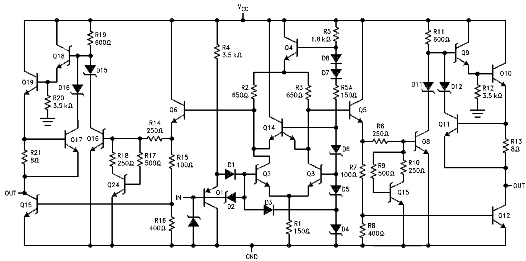
FIGURE 1. Equivalent Circuit
