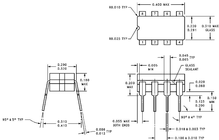
Ceramic Dual-In-Line Package (J) Order Number DS9638MJ/883 NS Package Number J08A
