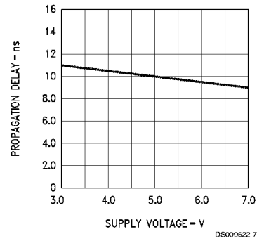
FIGURE 4. Typical Delay Characteristics
