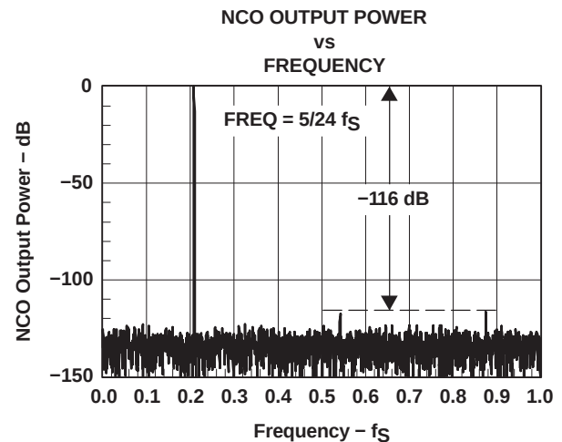
b) Spectrum With Dither (Tuned to Same Frequency)
