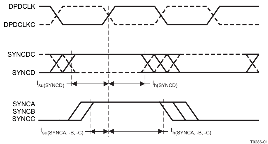
Figure 11. DPD Clock and Fast Sync Timing Specifications
