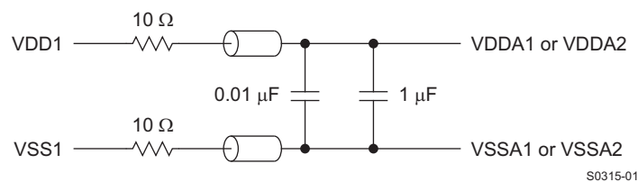
Figure 8. Recommended Filter for VDDA1, VDDA2 Power
