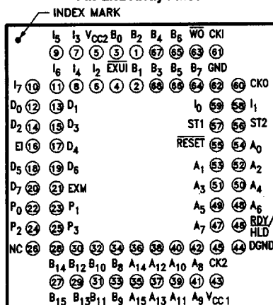
Pin Grid Array Pinout
