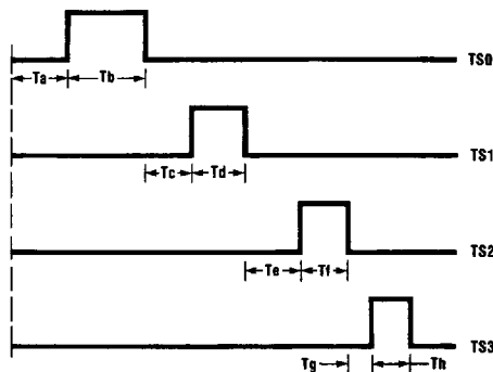
FIGURE 23. Synchronous Pulse Generation
