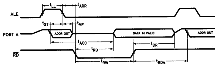
FIGURE 5. Read Cycle
