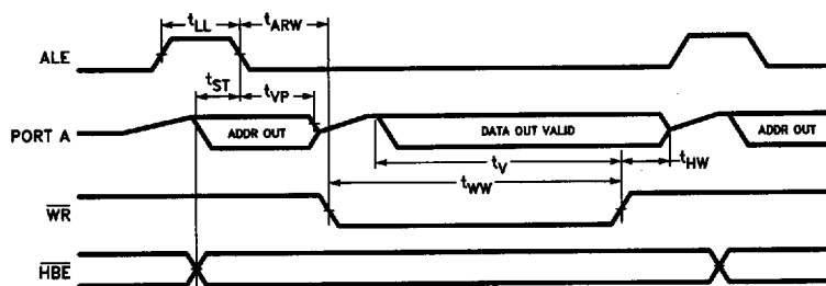
FIGURE 4. Write Cycle
