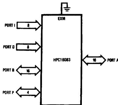
FIGURE 15. Single-Chip Mode
