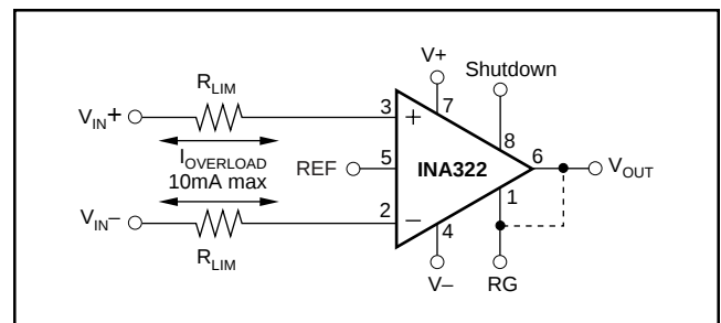
FIGURE 7. Input Protection.
