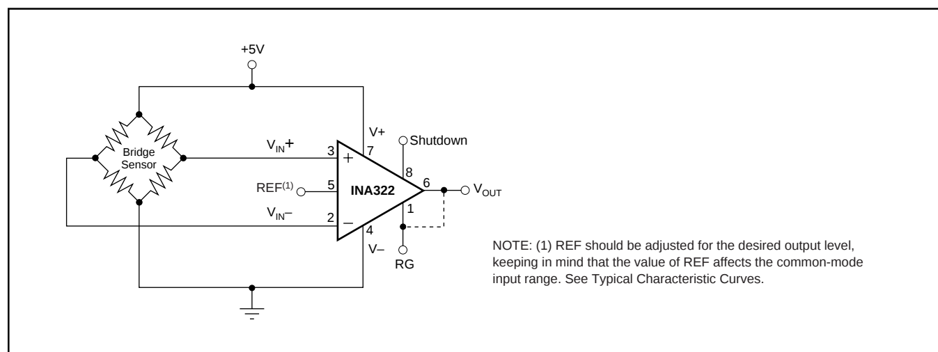
FIGURE 2. Bridge Amplifier of the INA322.
