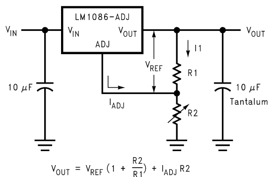
Figure 19. Basic Adjustable Regulator
