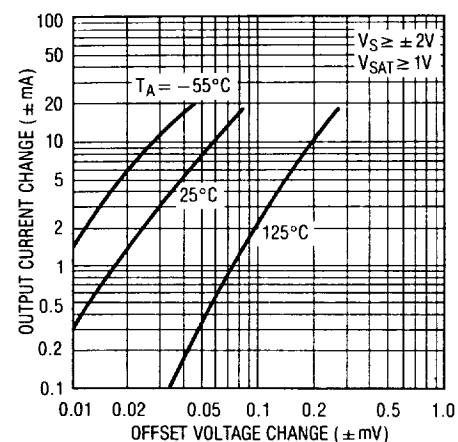
Transconductance
