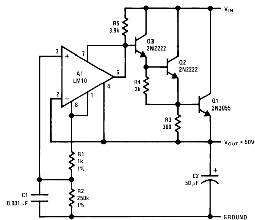
Figure 50. Precision Regulator
