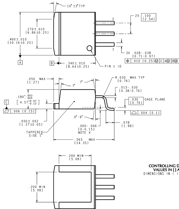
3-Lead TO-263 NS Package Number TS3B
