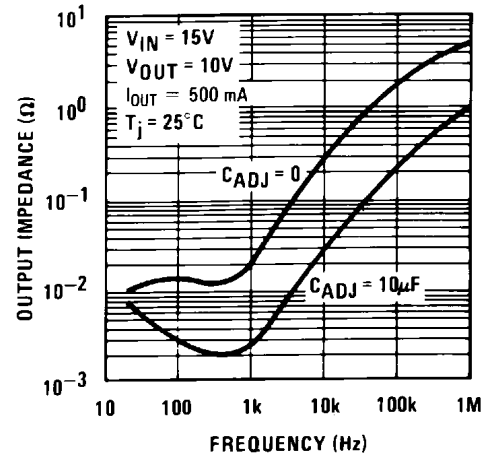
Output Impedance
