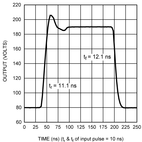
FIGURE 5. LM2422 Pulse Response
