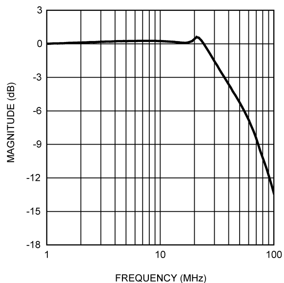
FIGURE 6. Bandwidth
