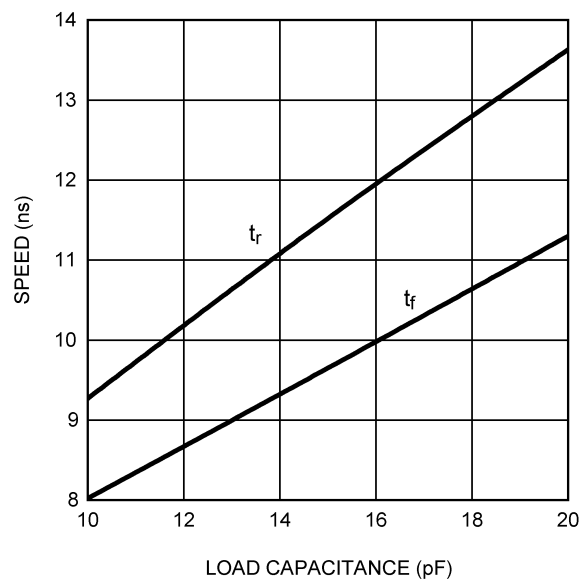
FIGURE 7. Speed vs Load Capacitance
