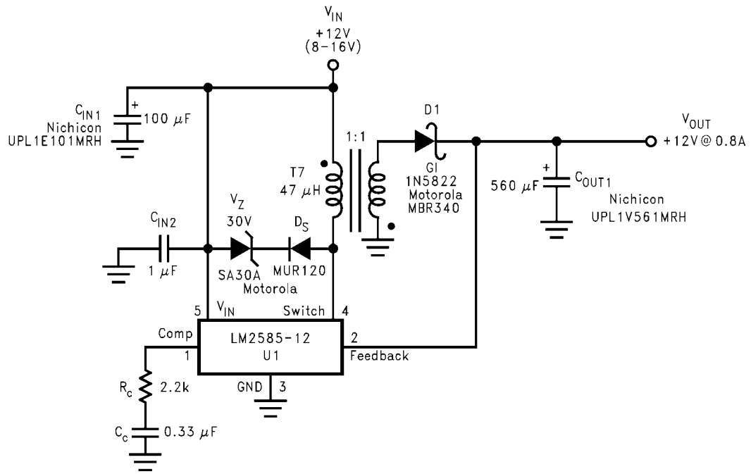
FIGURE 9. Single-Output Flyback Regulator
