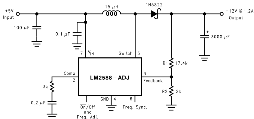
Figure 57. Boost Regulator
