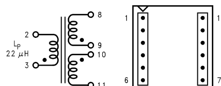
Figure 34. T2 - Top View Coilcraft Q4436-B (Surface Mount)
