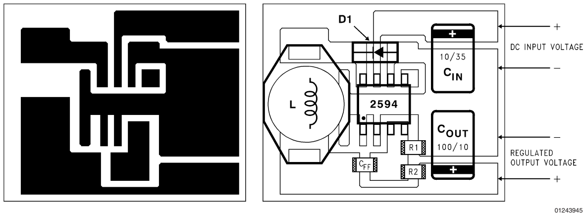
TYPICAL SURFACE MOUNT PC BOARD LAYOUT, ADJUSTABLE OUTPUT (2X SIZE)
