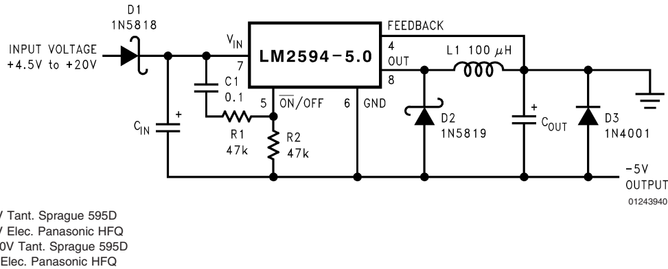
FIGURE 25. Inverting -5V Regulator with Delayed Startup
