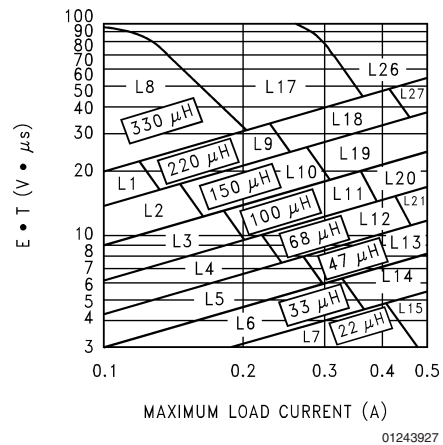
FIGURE 7. LM2594/LM2594HV-ADJ
