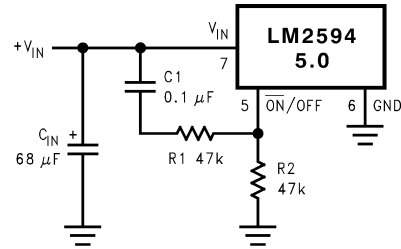
FIGURE 21. Delayed Startup
