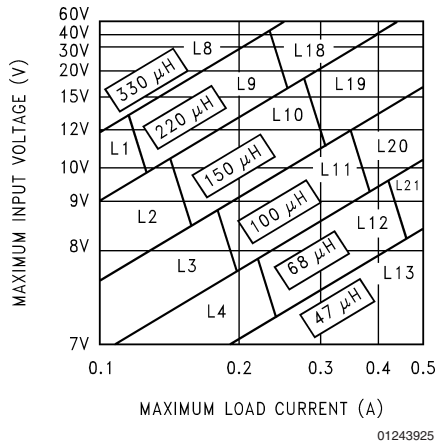
FIGURE 5. LM2594/LM2594HV-5.0
