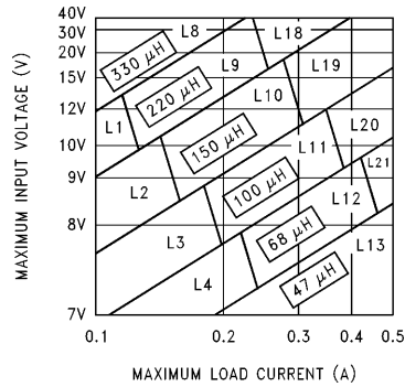
FIGURE 6. LM2594-5.0
