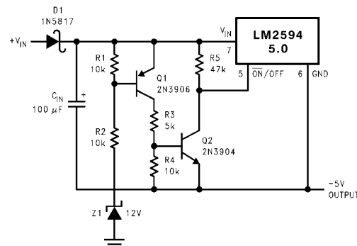
FIGURE 23. Undervoltage Lockout for Inverting Regulator
