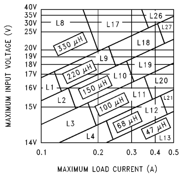
FIGURE 7. LM2594-12
