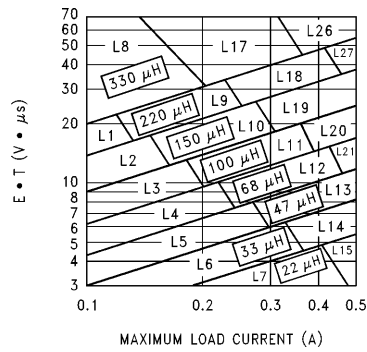
FIGURE 8. LM2594-ADJ
