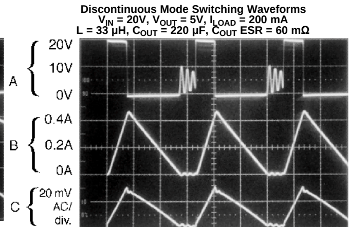
Figure 17. Horizontal Time Base: 2 \mu\text{s}/\text{div} .
