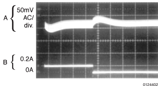
Load Transient Response for Discontinuous Mode V_{\text{IN}} = 20\text{V} , V_{\text{OUT}} = 5\text{V} , I_{\text{LOAD}} = 100\text{ mA to } 200\text{ mA} L = 33\text{ }\mu\text{H} , C_{\text{OUT}} = 220\text{ }\mu\text{F} , C_{\text{OUT}} \text{ ESR} = 60\text{ m}\Omega
