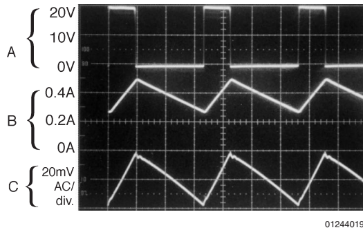
Continuous Mode Switching Waveforms V_{\text{IN}} = 20\text{V} , V_{\text{OUT}} = 5\text{V} , I_{\text{LOAD}} = 400\text{ mA} L = 100\text{ }\mu\text{H} , C_{\text{OUT}} = 120\text{ }\mu\text{F} , C_{\text{OUT}} \text{ ESR} = 140\text{ m}\Omega
