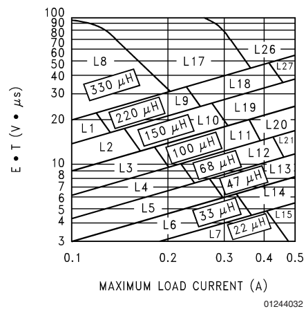
FIGURE 6. LM2597/LM2597HV-ADJ
