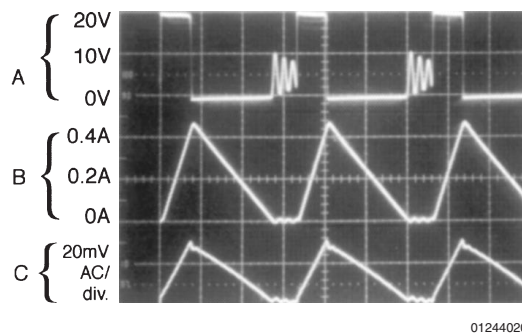
Discontinuous Mode Switching Waveforms V_{\text{IN}} = 20\text{V} , V_{\text{OUT}} = 5\text{V} , I_{\text{LOAD}} = 200\text{ mA} L = 33\text{ }\mu\text{H} , C_{\text{OUT}} = 220\text{ }\mu\text{F} , C_{\text{OUT}} \text{ ESR} = 60\text{ m}\Omega
