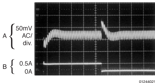
Load Transient Response for Continuous Mode V_{\text{IN}} = 20\text{V} , V_{\text{OUT}} = 5\text{V} , I_{\text{LOAD}} = 200\text{ mA to } 500\text{ mA} L = 100\text{ }\mu\text{H} , C_{\text{OUT}} = 120\text{ }\mu\text{F} , C_{\text{OUT}} \text{ ESR} = 140\text{ m}\Omega
