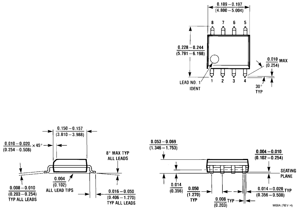
8-Lead (0.150" Wide) Molded Small Outline Package, Order Number LM2597M-3.3, LM2597M-5.0, LM2597M-12 or LM2597M-ADJ LM2597HVM-3.3, LM2597HVM-5.0, LM2597HVM-12 or LM2597HVM-ADJ NS Package Number M08A
