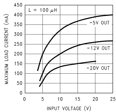
FIGURE 30. Maximum Load Current for Inverting Regulator Circuit
