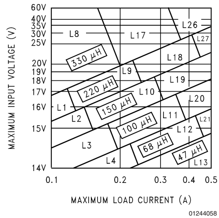
FIGURE 5. LM2597/LM2597HV-12
