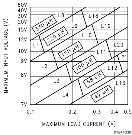
FIGURE 4. LM2597/LM2597HV-5.0
