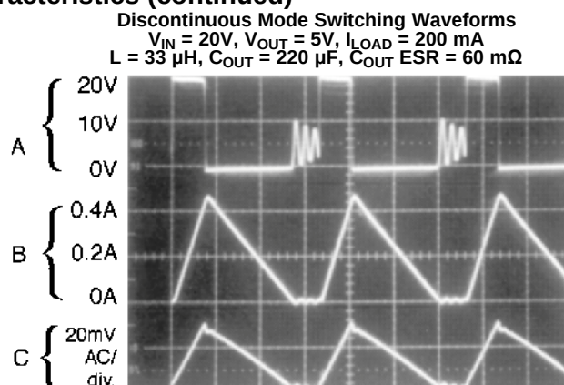
Figure 23. Horizontal Time Base: 2 \mu\text{s} /div.
