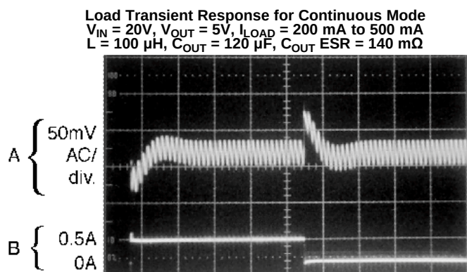
Figure 22. Horizontal Time Base: 2 \mu\text{s}/\text{div} .
