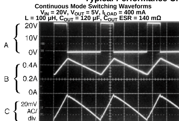
Figure 22. Horizontal Time Base: 2 \mu\text{s}/\text{div} .
