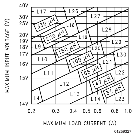
FIGURE 6. LM2598-12
