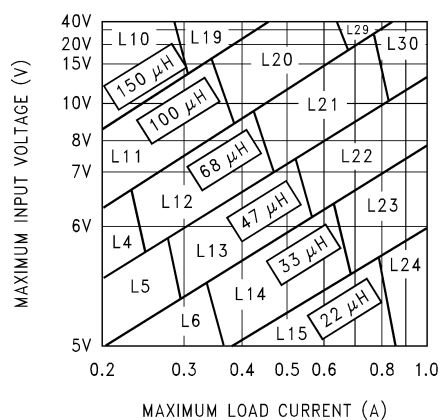
FIGURE 4. LM2598-3.3
