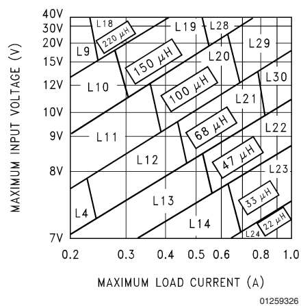
FIGURE 5. LM2598-5.0
