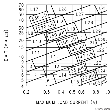
FIGURE 7. LM2598-ADJ
