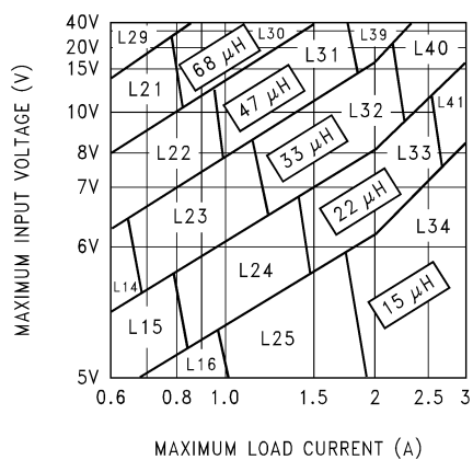
FIGURE 4. LM2599-3.3
