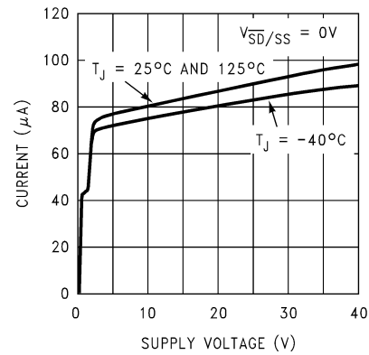
Shutdown Quiescent Current
