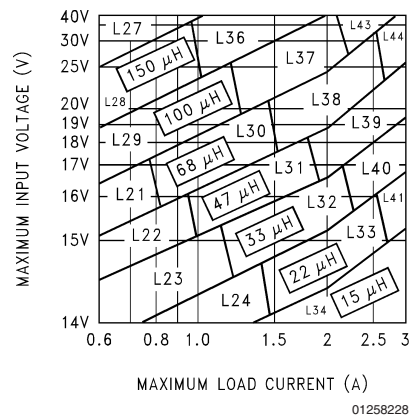
FIGURE 6. LM2599-12
