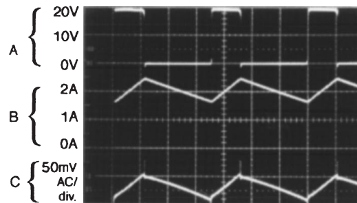
Continuous Mode Switching Waveforms V_{IN} = 20V , V_{OUT} = 5V , I_{LOAD} = 2A L = 32 \mu H , C_{OUT} = 220 \mu F , C_{OUT} ESR = 50 m\Omega
