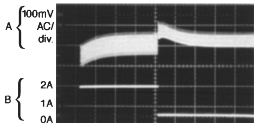
Load Transient Response for Discontinuous Mode V_{IN} = 20V , V_{OUT} = 5V , I_{LOAD} = 500 mA to 2A L = 10 \mu H , C_{OUT} = 330 \mu F , C_{OUT} ESR = 45 m\Omega
