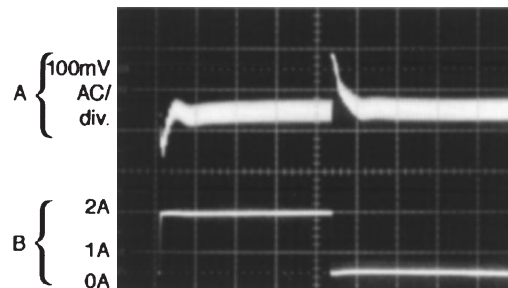
Load Transient Response for Continuous Mode V_{IN} = 20V , V_{OUT} = 5V , I_{LOAD} = 500 mA to 2A L = 32 \mu H , C_{OUT} = 220 \mu F , C_{OUT} ESR = 50 m\Omega
