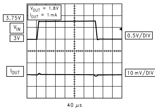
LDO Line Transient Response
