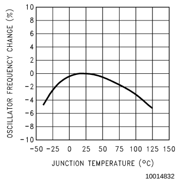
Normalized Oscillator Frequency vs. Junction Temperature
