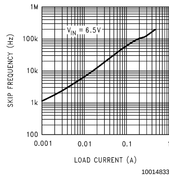
CH1 Skip Frequency vs Load Current
