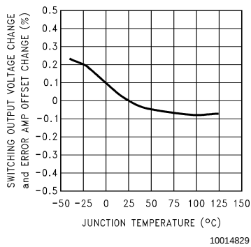
Normalized Error Amplifier Offset vs Junction Temperature
