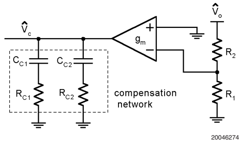
FIGURE 12. Compensation Network
