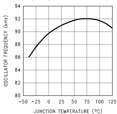
Oscillator Frequency vs Junction Temperature
