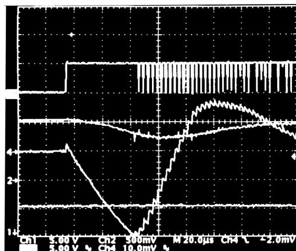
CH1: PGOOD, CH2: Vo, CH3: LDRV, CH4: I_L (1A/div) Output 1V @ 0A, VIN = 10V, L = 10μH, f = 300kHz
