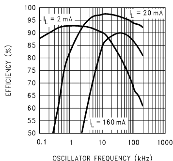
Efficiency vs Oscillator Frequency
