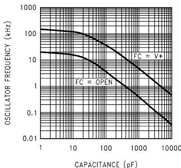
Oscillator Frequency vs External Capacitance
