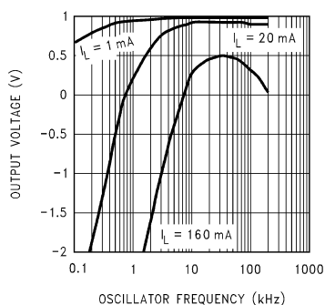
Output Voltage vs Oscillator Frequency
