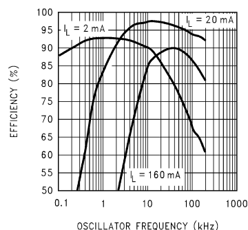
Efficiency vs Oscillator Frequency
