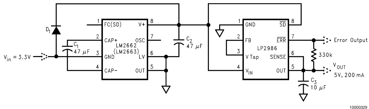
FIGURE 9. Generating +5V from +3.3V Input Voltage
