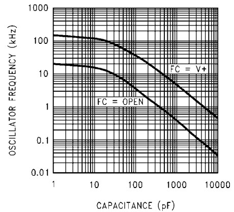
Oscillator Frequency vs External Capacitance
