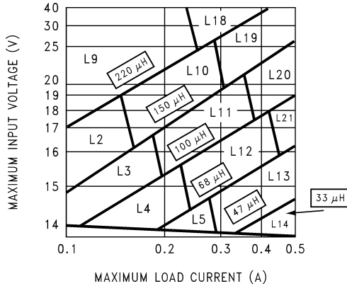
Figure 26. LM2671-12
