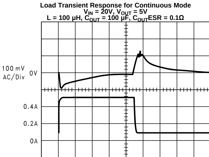
Figure 18. Horizontal Time Base: 1 \mu\text{s}/\text{div}
