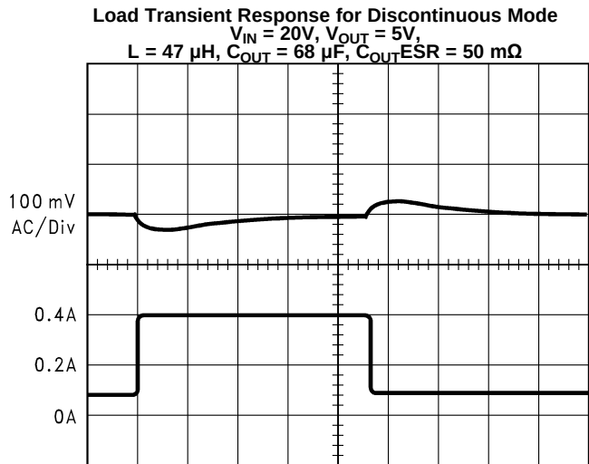
Figure 19. Horizontal Time Base: 1 \mu\text{s}/\text{div}
