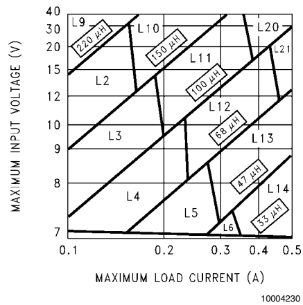
FIGURE 5. LM2671-5.0
