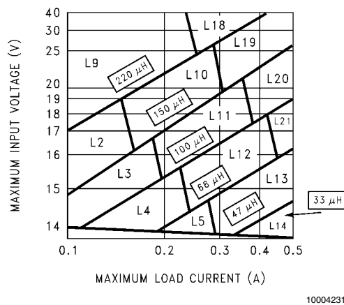
FIGURE 6. LM2671-12
