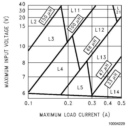
FIGURE 4. LM2671-3.3
