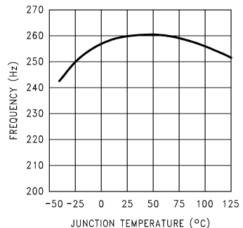
Switching Frequency
