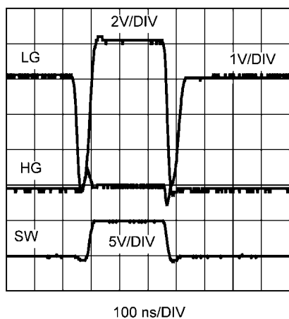
Switch Waveforms
