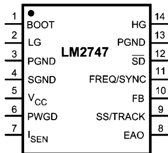
20150990 14-Lead Plastic TSSOP \theta_{JA} = 155^{\circ}\text{C/W} NS Package Number MTC14
