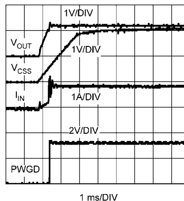
Start-Up (Full-Load)
