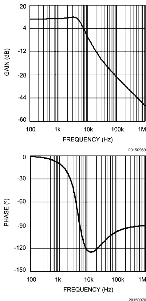
FIGURE 14. Power Stage Gain and Phase
