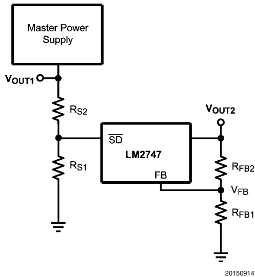
FIGURE 6. Sequencing Circuit
