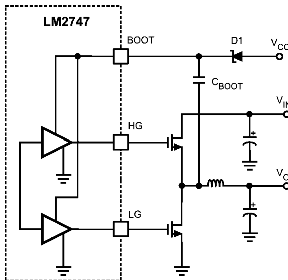
FIGURE 9. Basic Charge Pump (Bootstrap)
