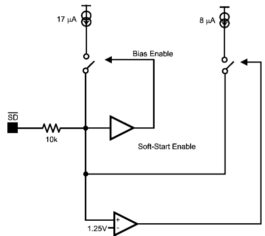
FIGURE 8. \overline{\text{SD}} Pin Logic
