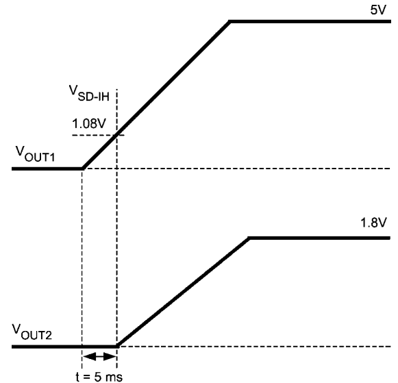
FIGURE 7. Delay for Sequencing
