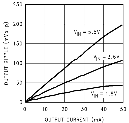
Output Voltage Ripple vs. Output Current
