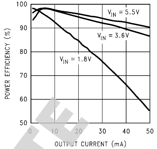
Power Efficiency vs. Load Current
