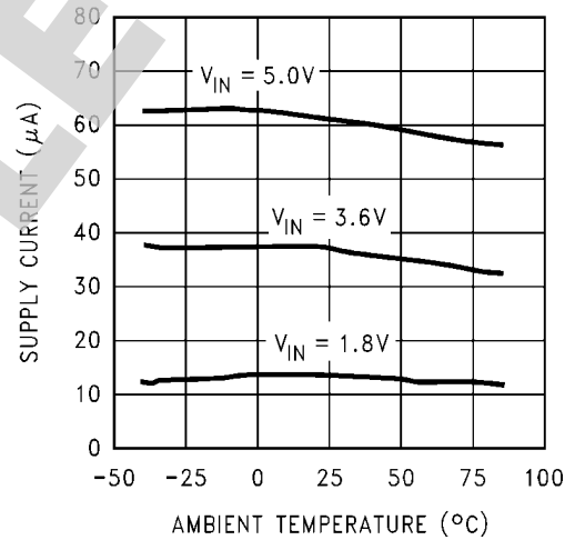
Supply Current vs. Temperature ( I_{OUT} = 0 )
