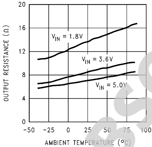
Output Resistance vs. Temperature ( I_{OUT} = 10\text{mA} )
