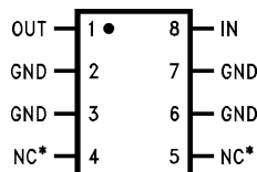
8-Pin Surface Mount
