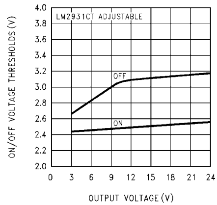
On/Off Threshold
