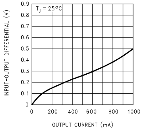
Dropout Voltage
