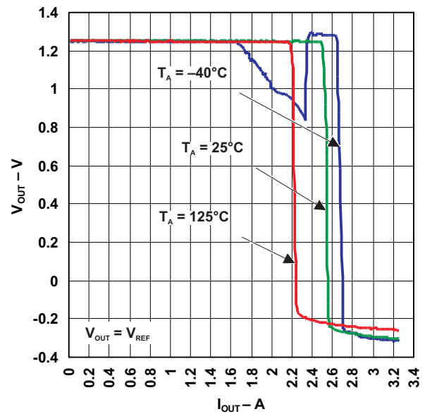
LOAD REGULATION
