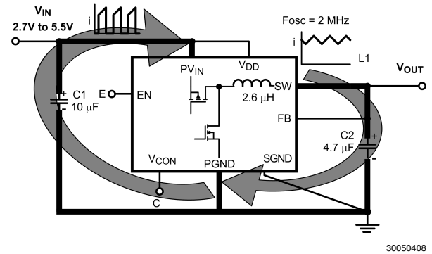
FIGURE 4. Current Loop
