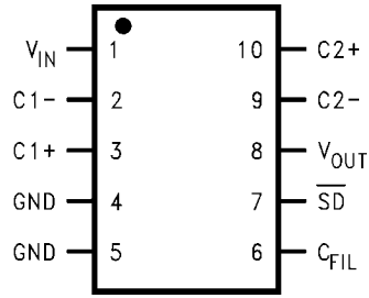
Top View MSOP-10 Pin Package See NS Package Number MM
