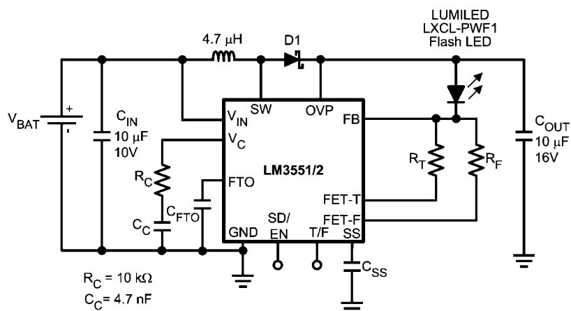
LUMILED LXCL-PWF1 R_T = 5.6\Omega , R_F = 2.2\Omega I_{TORCH} = 200\text{mA} , I_{FLASH} = 700\text{mA}
