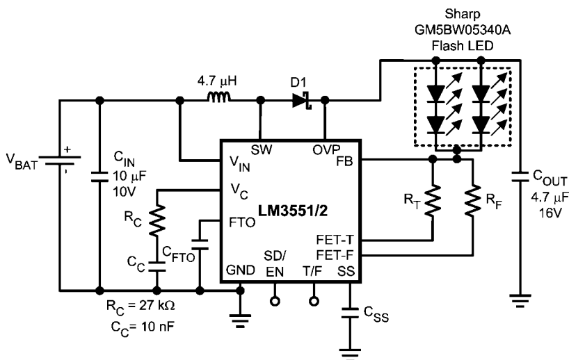
SHARP GM5BW05340A R_T = 17\Omega , R_F = 6.5\Omega I_{TORCH} = 75\text{mA} , I_{FLASH} = 250\text{mA}
