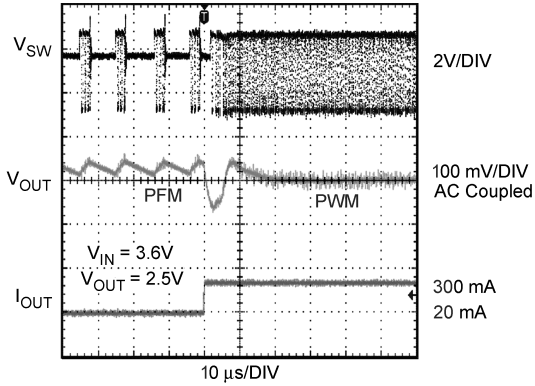
Mode Change by Load Transients V_{OUT} = 2.5V (PFM to PWM)
