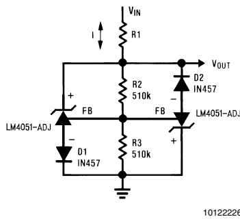
FIGURE 7. Bidirectional Clamp ±2.4V
