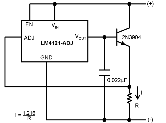
Two Terminal Constant Current Source
