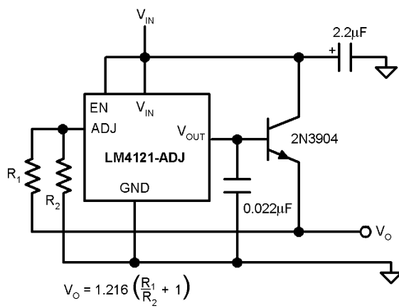
100mA Quasi-LDO Regulator
