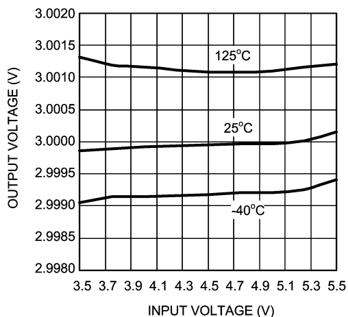
Line Regulation
