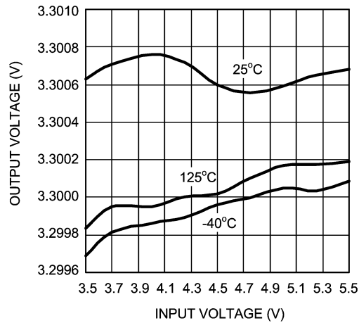
Line Regulation
