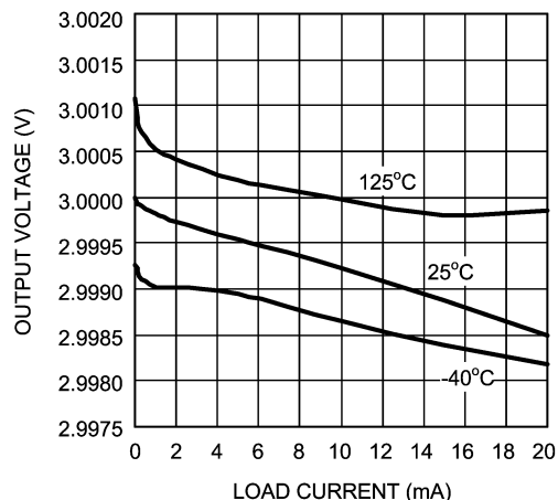
Load Regulation
