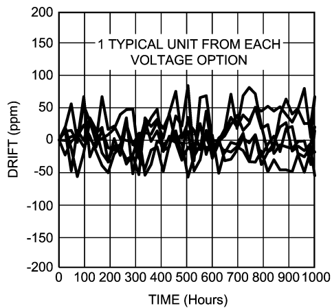
Typical Long Term Stability
