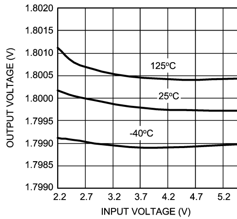
Line Regulation
